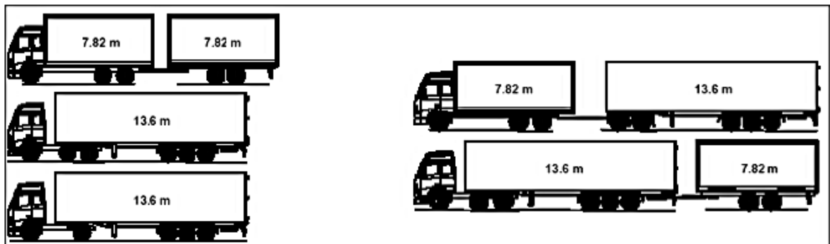
Figure 1 Typical freight truck and trailer combinations in Sweden and Finland [10].
