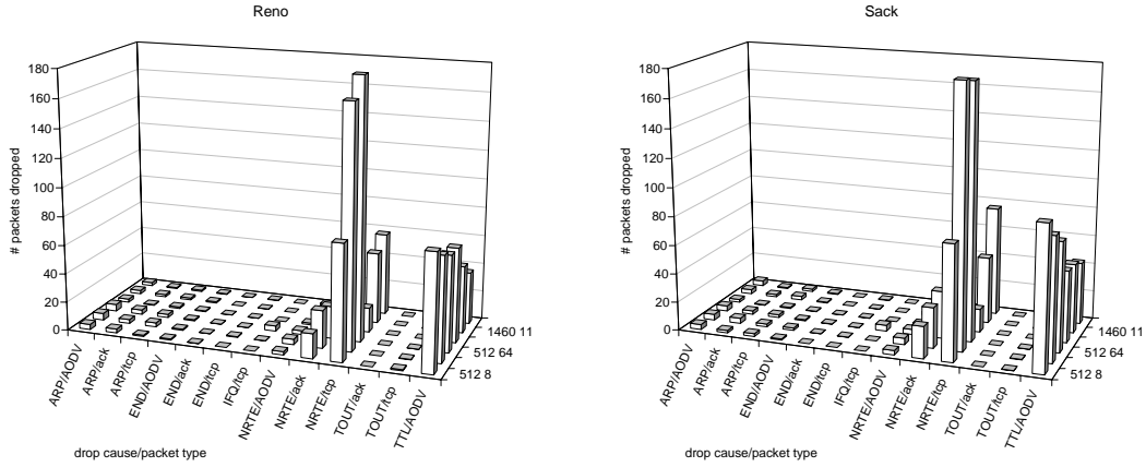
Figure 34: Packets dropped, average speed 10 m/s and AODV.
