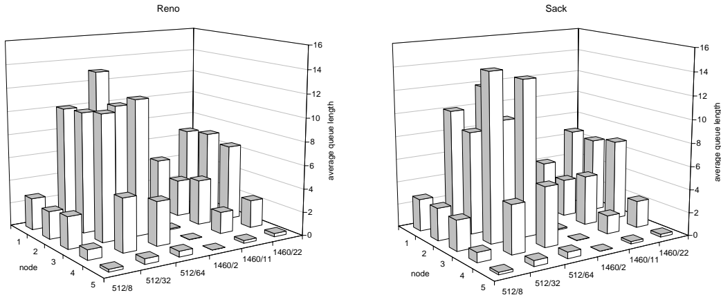
Figure 17: Average queue length using AODV.
