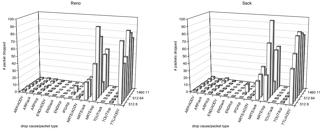
Figure 32: Packets dropped, average speed 2 m/s and AODV.
