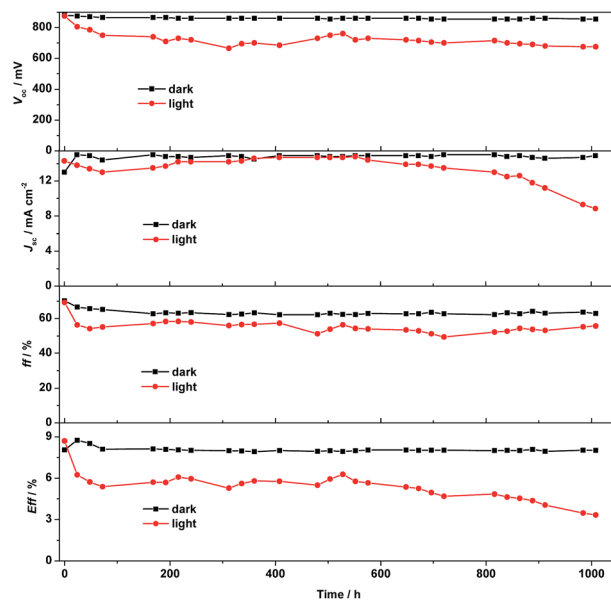
Fig. 8 The stability of DSSCs fabricated using the [\text{Cu}(\text{bpye})_2](\text{PF}_6)_2 redox couple studied under dark and under light soaking at 40^\circ\text{C} for 1000 h.
