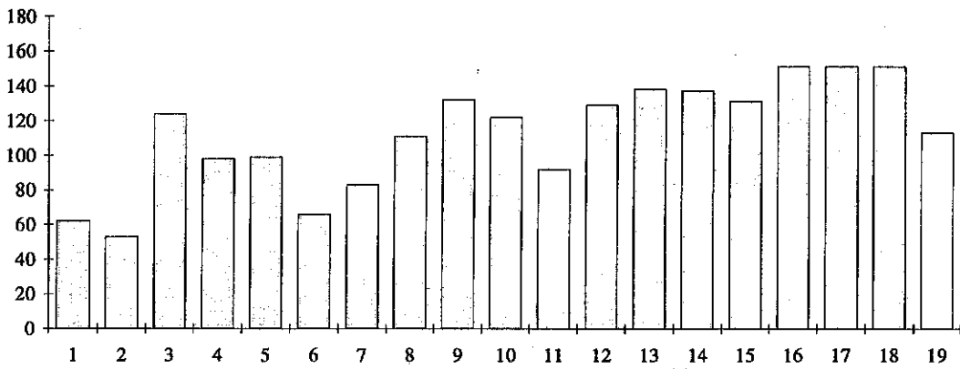
Diagram 17. Measured head peak acceleration (g) for type C helmet.
