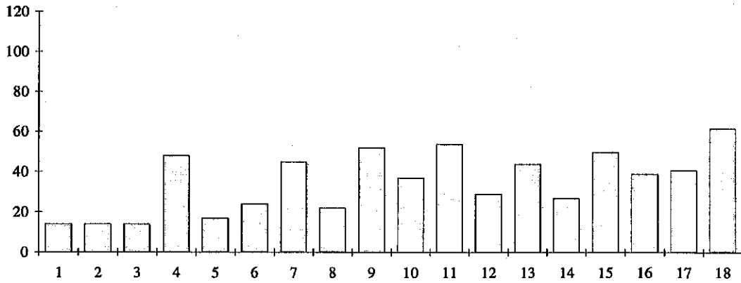
Diagram 16. Measured chin strap peak forces (N) for type C helmet.
