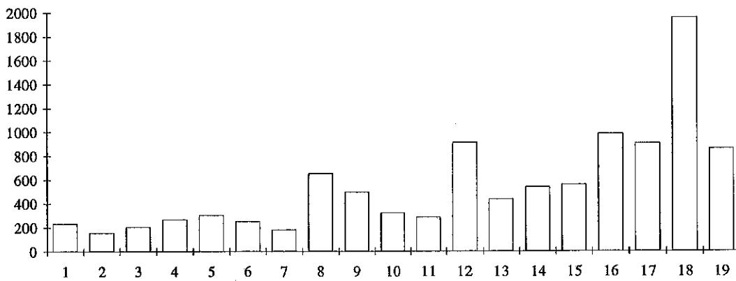
Diagram 15. Calculated head injury criterion (HIC) for type B helmet.
