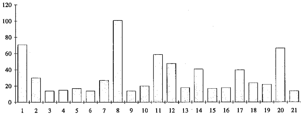
Diagram 1. Measured chin strap peak forces (N) at 23 km/h carriage speed.
