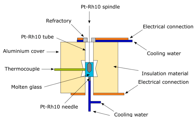
Fig. 1. Rotational rheometer setup.
