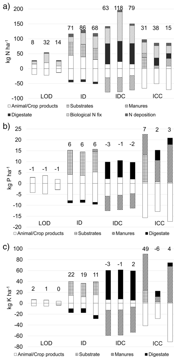
Fig. 2 Farm-gate budget for a nitrogen (N), b phosphorus (P), and c potassium (K) in the three study years (2015–2017) on the low-input dairy farm with on-farm biogas reactor (LOD), the intensive dairy (ID) farm with on-farm biogas reactor, the intensive dairy farm with central biogas plant (IDC), and the intensive crop farm importing digestate (ICC). Values above bars indicate net surplus/depletion. Animal products include feed, milk, animals, and bedding. Crop products include crops and seed
