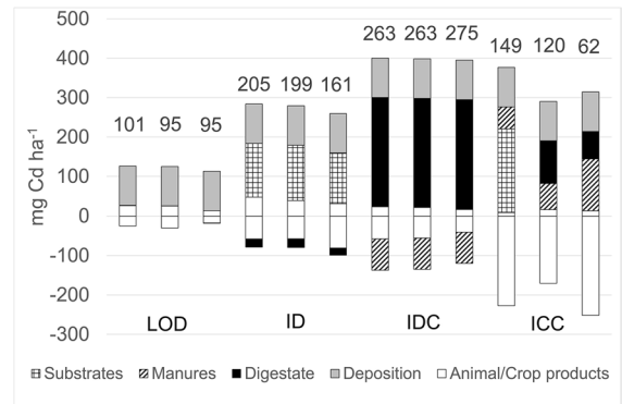
Fig. 3 Cadmium (Cd) farm-gate budget in the three study years (2015–2017) on the low-input dairy farm with on-farm biogas reactor (LOD), the intensive dairy farm with on-farm biogas reactor (ID), the intensive dairy farm with central biogas plant (IDC), and the intensive crop farm importing digestate (ICC). Values above bars indicate net surplus/depletion. Animal products include feed, milk, animals, and bedding. Crop products include crops and seed
