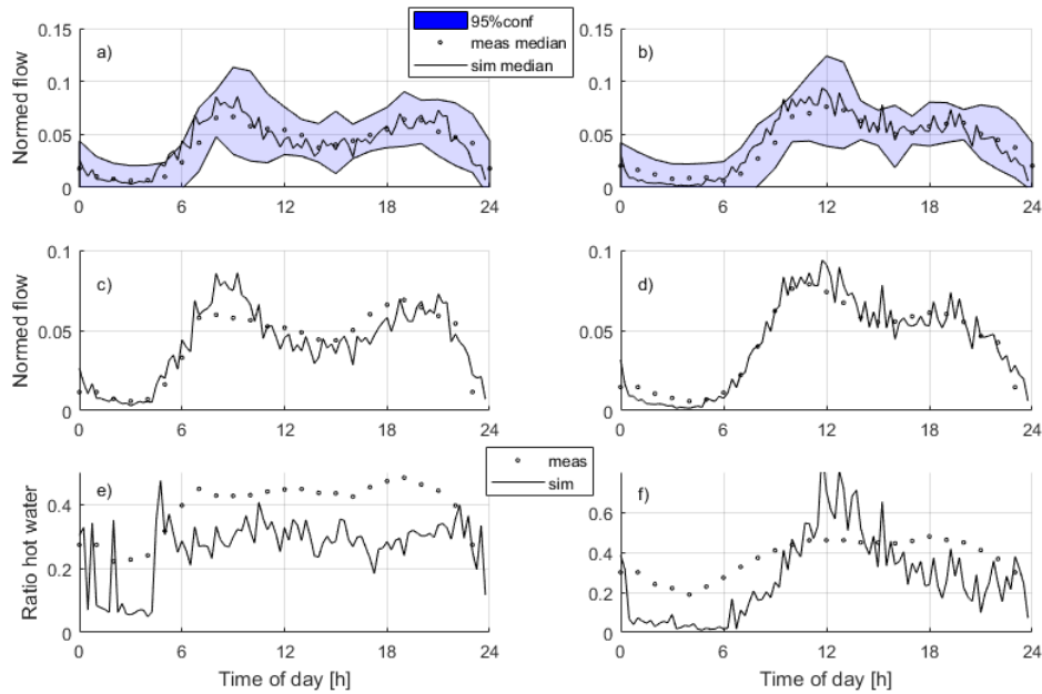
Figure 3. Normed simulated median flow compared to median values and measured 95 percent confidence intervals for water demand curves from Nikell (1994) for workday (a) and weekend (b), as well as normed simulated median flow compared to normed measured median flow of tap water (workday (c) and weekend (d)) as well as the fraction of water use that is hot water (workday (e), weekend (f)) from measurements in Karlstad, Sweden.
