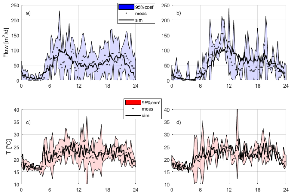
Figure 2. Simulated median flow compared to measured median flow and 95 percent confidence intervals for measurements. Flow measurements performed in Linköping, Sweden.
