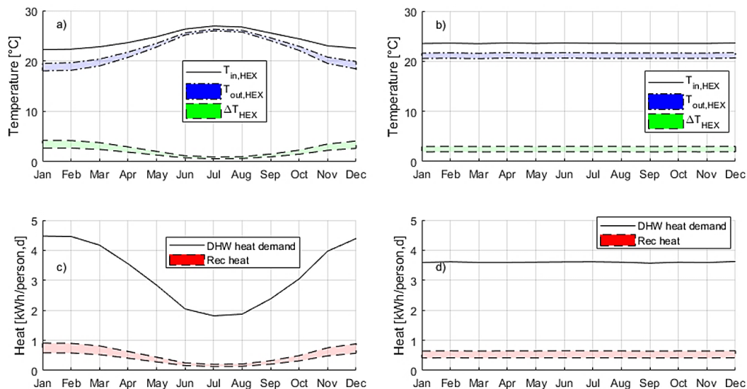
Figure 5. Wastewater temperature before and after heat exchanger as well as temperature drop for Scenarios 1 (a) and 2 (b), monthly mean recovered heat energy and mean monthly domestic hot water heat energy demand for Scenarios 1 (c) and 2 (d). Intervals represent results for the specified interval for \epsilon_{\text{hex}} (0.335 – 0.52).
