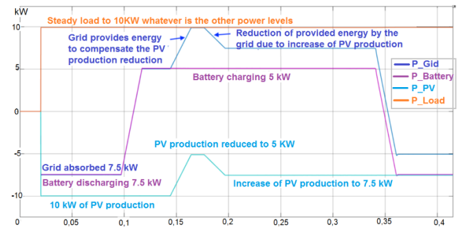
Figure 3. Active power flow in grid connected mode.
