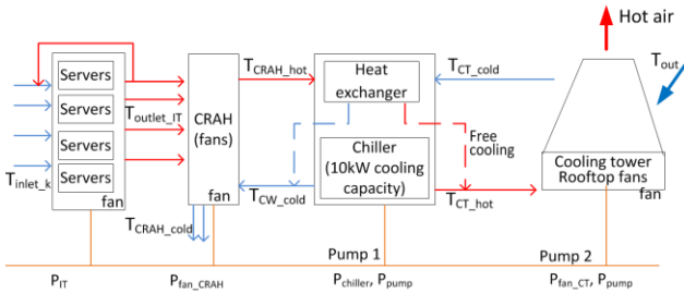
Figure 1. Overview of the data center model.
