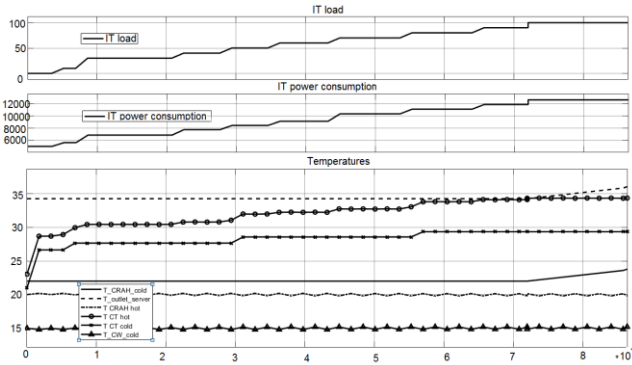
Figure 4. Data center with the 6-core servers (without frequency scaling): temperatures throughout server room and cooling system.
