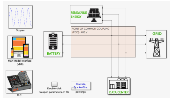
Figure 2. DMI data center microgrid model (Matlab Simulink).
